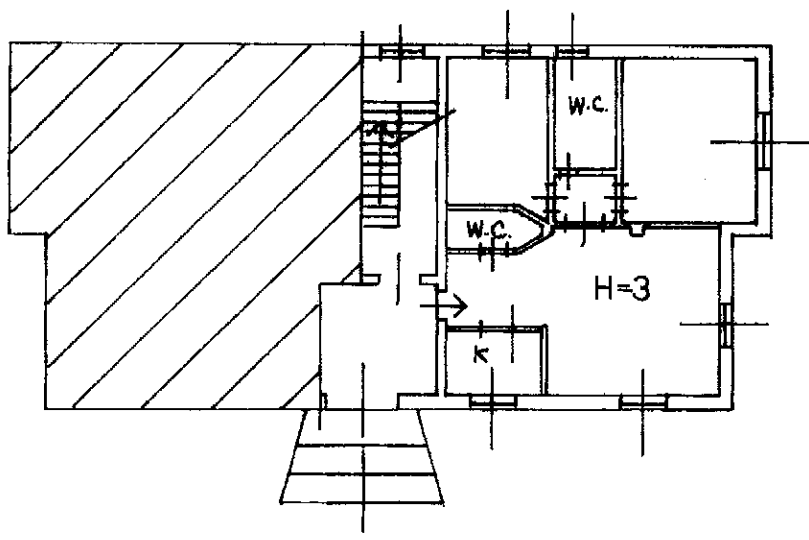
PIANO TERRENO
